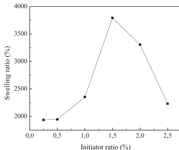
Fig. 6. The relationship between the swelling ratio with the initiator ratio.
